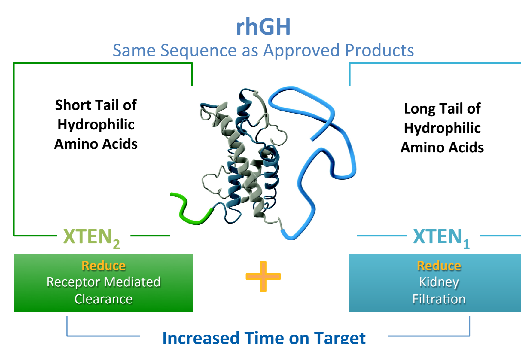
Figure 1. Somavaratan Structure-Function
